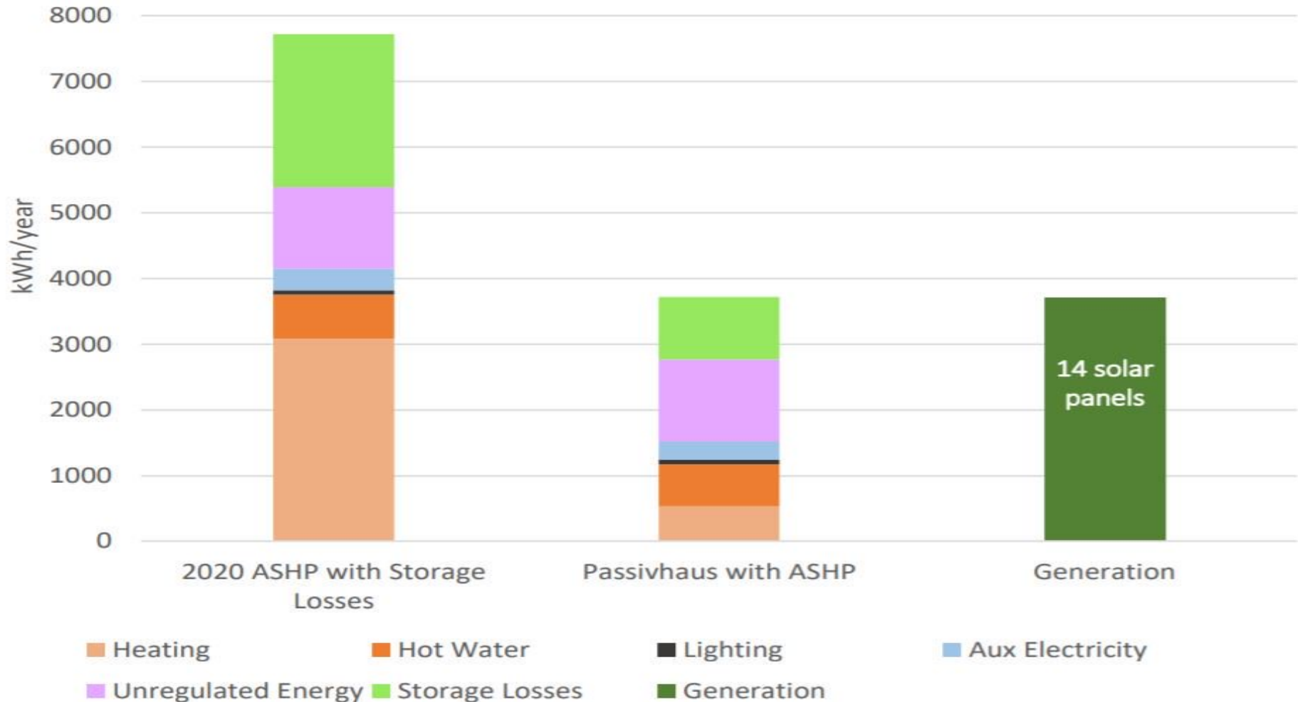
Figure 4 - Average new build energy demand vs Passivhaus
